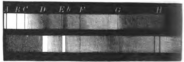
FIG. 6.—Absorption and fluorescing spectrum of naphthalin red.
